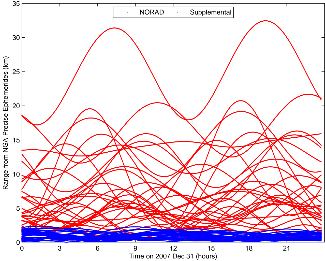
Comparison of NORAD and Supplemental TLEs
